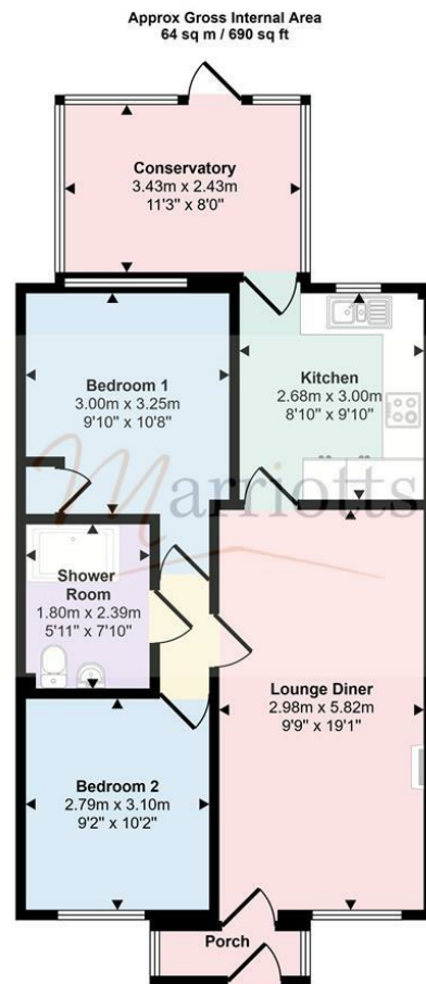
Floorplan
